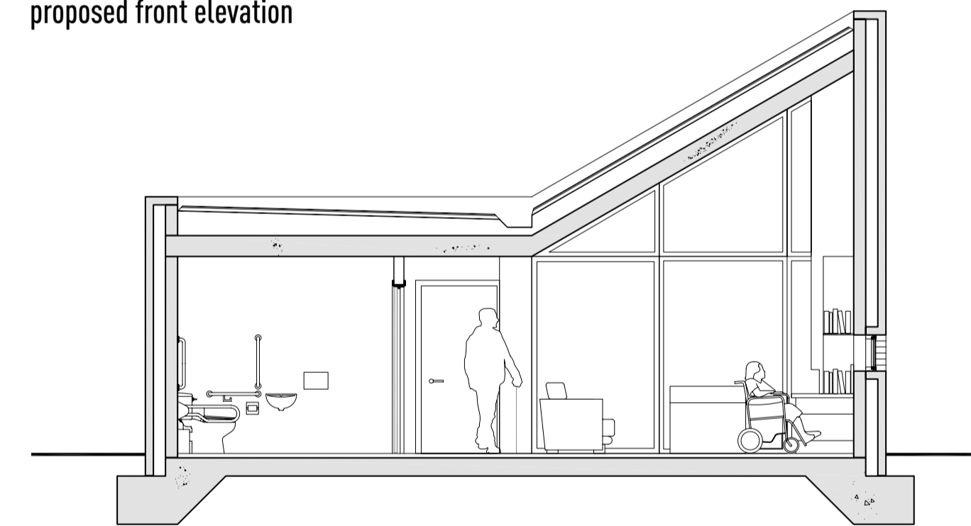
cross section
